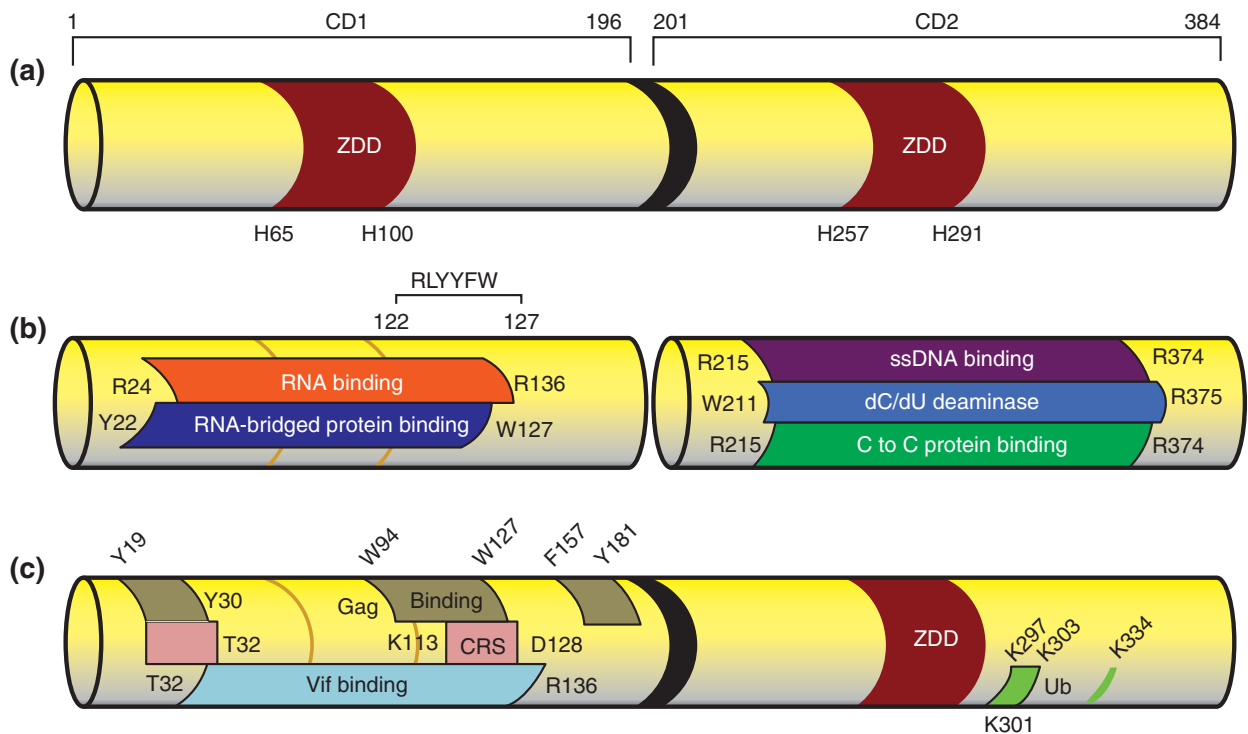
FIGURE 3 | Important functional domains of A3G. (a) Schematic of full-length A3G protein highlighting the regions comprising the two ZDDs (N-terminal ZDD spans residues 65–100, C-terminal ZDD spans residues 257–291). (b) Separation of A3G's N- and C-termini to highlight the characteristics and functions of each half of the protein. The N-terminal half of A3G is required for both RNA binding (residues 24–136) and RNA bridged A3G multimerization (residues 22–127). Residues 122–127 have been suggested to mediate N-terminal dimerization of A3G in a head-to-head fashion. The C-terminal portion of A3G is required for its ssDNA binding and deaminase activity (residues 215–374 and 211–375, respectively). The C-terminus is also responsible for A3G tail-to-tail dimerization (residues 215–374). (c) Representation of the A3G domains required for interaction with viral proteins and cellular localization. The cytoplasmic retention signal (CRS) of A3G is located in the N-terminal half of the protein, requiring residues 19–32 and 113–128. A3G incorporation with virions requires an interaction with the HIV Gag protein, which is facilitated by multiple regions of the N-terminal domain (residues 19–30, 94–127, 157–181). In addition to Gag binding, the N-terminal domain of A3G has been shown to interact with HIV Vif (residues 32–136). Upon binding to Vif, A3G is ubiquitinated (Ub) at C-terminal lysine residues, including K297, K301, K303, and K334.
