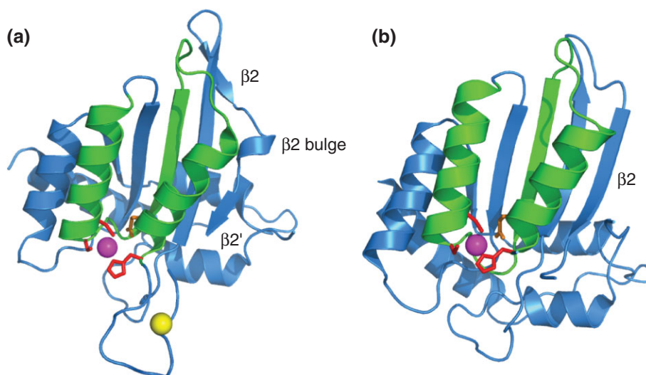
FIGURE 2 | Representative APOBEC crystal structures. Diagram of a representative crystal structure of (a) the C-terminal Z1-type CDA of A3G (PDB 3IR2) at 2.25 Å resolution 73 and (b) the C-terminal Z-2 type CDA of A3F (PDB 4IOU) at 2.75 Å resolution. 74 The \alpha\beta\alpha supersecondary structural element (green) is shown embedded within the core CDA fold, comprising the five-stranded, mixed \beta -sheet surrounded by six \alpha -helices, typical of the A3 family. Sidechains of the conserved zinc-binding residues and proton-shuttling glutamic acid are illustrated in red and orange, respectively. The catalytic zinc ion is represented as a purple sphere. The additional non-catalytic zinc ion present in the A3G structure is represented by the yellow sphere; it is coordinated by four residues, two from each of adjacent subunits within the crystal and may be an artifact due to crystal packing. The \beta 2 bulge between \beta 2 and \beta 2' is present in the structure of the Z1-type CDA of the A3G C-terminal CDA (a), but is noticeably absent from the Z2-type CDA of the A3F C-terminal CDA (b).
