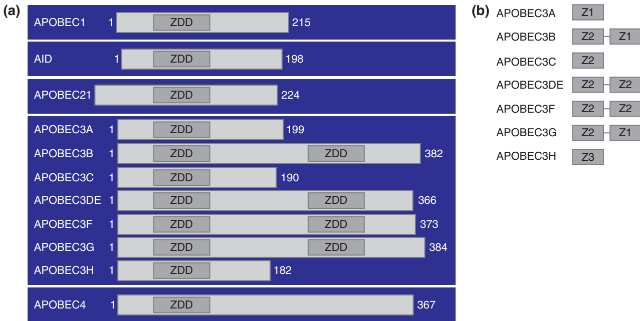
FIGURE 1 | The ZDD of the APOBEC family. (a) The ZDD sequence motif [(H/C)-x-E-x (25–30) -P-C-xx-C] is conserved throughout the APOBEC family of cytidine deaminases. Several APOBEC3 members (B, DE, F, and G) have two ZDD motifs in tandem on a single polypeptide. (b) The CDA domains of the A3 family members are subcategorized as Z1, Z2, or Z3 type according to additional conserved sequences within the ZDD motif.
